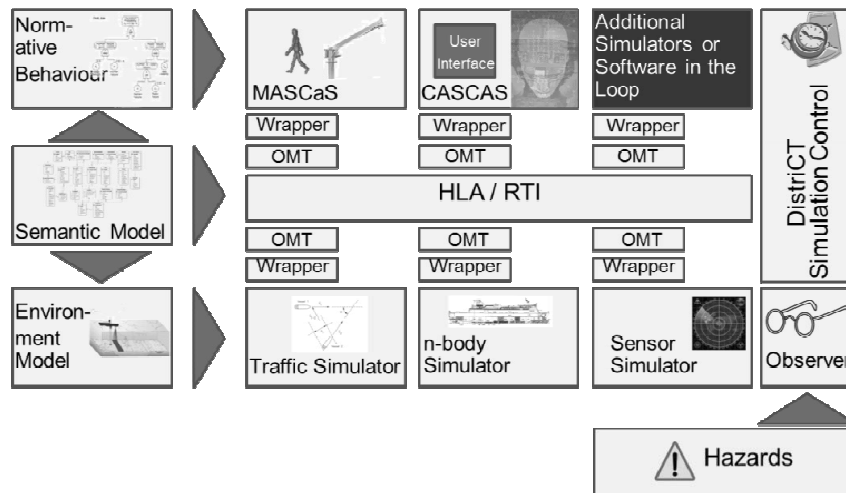
Figure 6 : HAGGIS Co-simulation Environment
